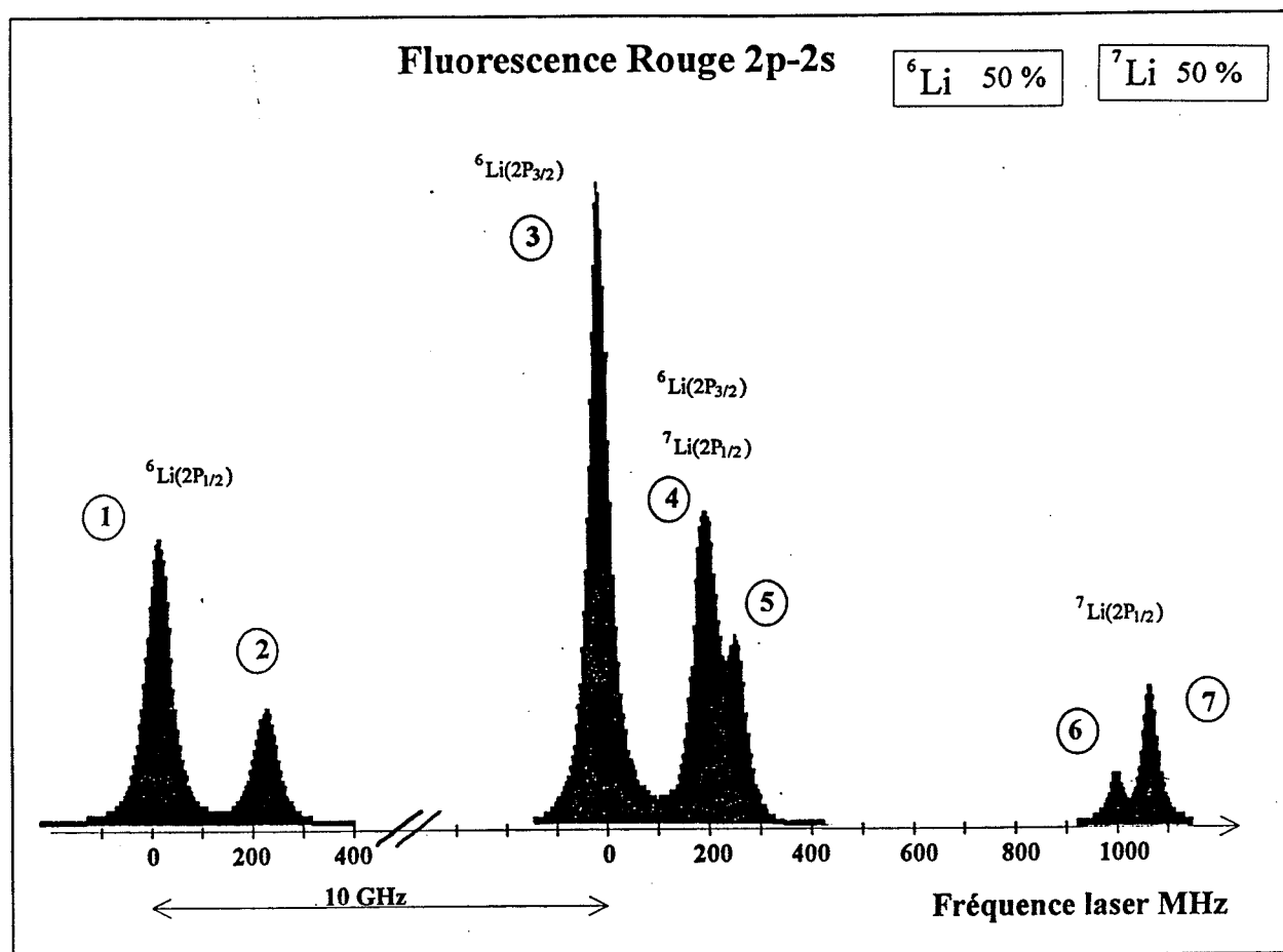
Figure 6.15: Avec mélange isotopique {}^7\text{Li} (50 %) et {}^6\text{Li} (50 %). Le laser I balaye la transition 2s→2p. Pic 1: {}^6\text{Li}[(2S(1/2), F'' = 3/2) \rightarrow 2P(1/2)] . Pic 2: {}^6\text{Li}[(2S(1/2), F'' = 1/2) \rightarrow 2P(1/2)] . Pic 3: {}^6\text{Li}[(2S(1/2), F'' = 3/2) \rightarrow 2P(3/2)] . Pic 4: {}^6\text{Li}[(2S(1/2), F'' = 1/2) \rightarrow 2P(3/2)] et {}^7\text{Li}[(2S(1/2), F'' = 2) \rightarrow (2P(1/2), F' = 1)] . Pic 5: {}^7\text{Li}[(2S(1/2), F'' = 2) \rightarrow (2P(1/2), F' = 2)] . Pic 6: {}^7\text{Li}[(2S(1/2), F'' = 1) \rightarrow (2P(1/2), F' = 1)] . Pic 7: {}^7\text{Li}[(2S(1/2), F'' = 1) \rightarrow (2P(1/2), F' = 2)] .
